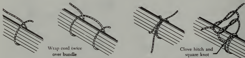
FIGURE 4-103. Tying a wire group or bundle.
